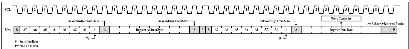
Figure 58 Reading from IS32LT3129
