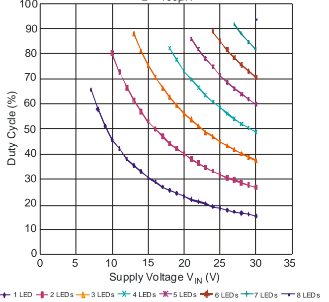
ZXLD1360 Duty Cycle L = 100μH
