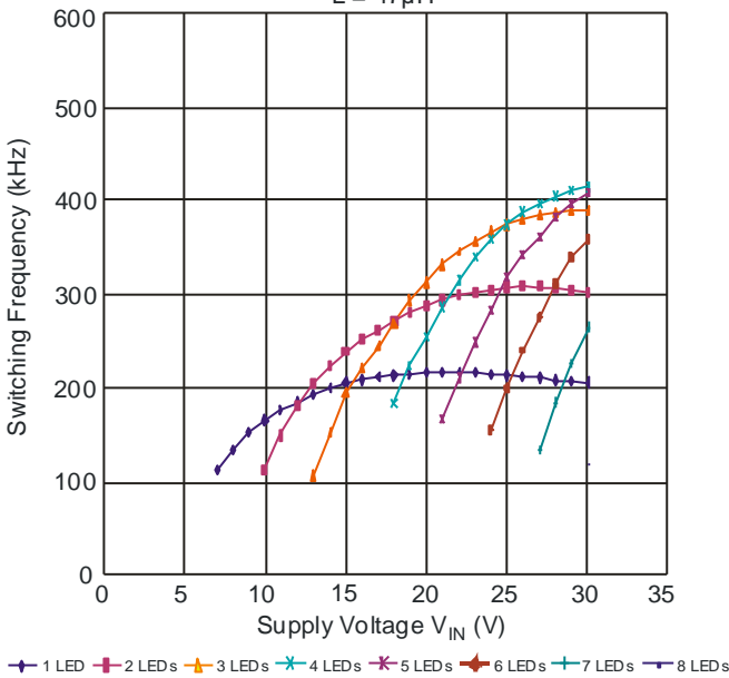
ZXLD1360 Switching Frequency L = 47μH
