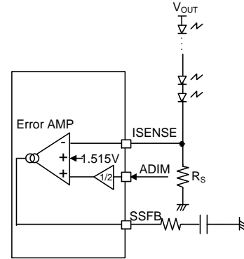
Figure 2. The ISENSE Pin Circuit Example
