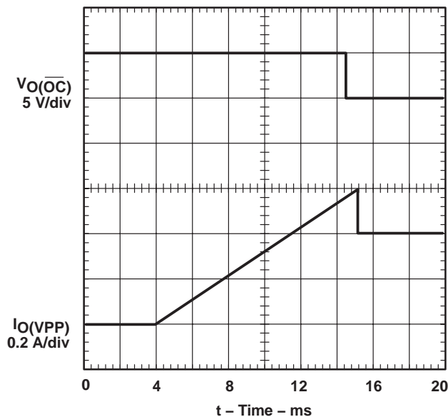
Figure 7. \overline{V_O} Response With Ramped Load on 12-V xVPP-Switch Output
