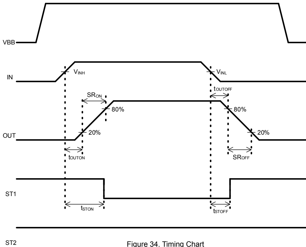
Figure 34. Timing Chart
