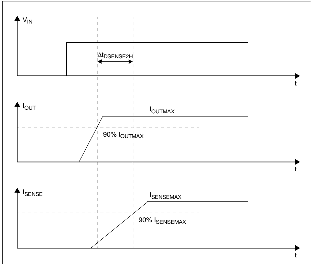
Figure 7. Switching characteristics
