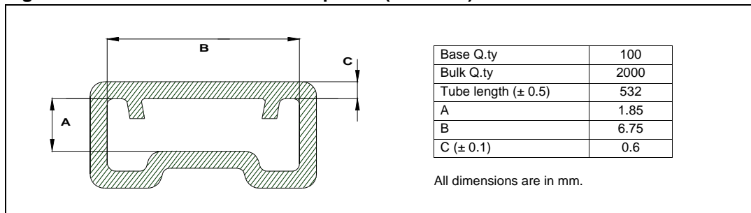
Figure 33. PowerSSO-12™ tube shipment (no suffix)
