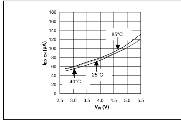
FIGURE 2-4: I_{DD\_ON} vs. V_{IN} .
