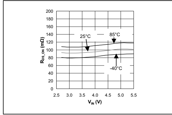
FIGURE 2-5: R_{DS\_ON} vs. V_{IN} .
