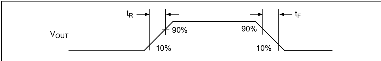
FIGURE 1-2: Output Rise and Fall Times.
