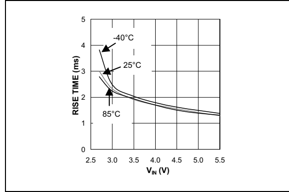
FIGURE 2-6: Output Rise Time vs. V_{IN} .
