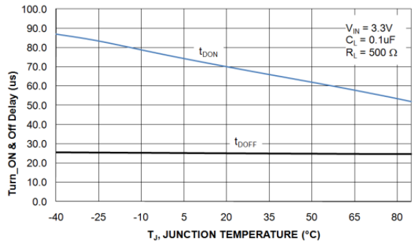
Figure 12. V_{OUT} Turn-On/Turn-Off Delays vs. Temperature ( R_L = 500 \Omega )
