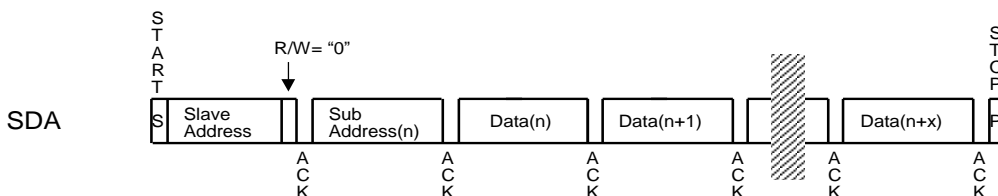
Figure 70. Data Transfer Sequence in I 2 C-Bus control mode
