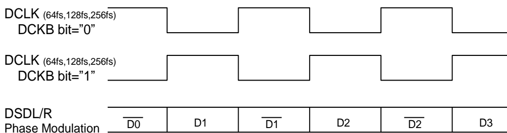
Figure 46. DSD mode Timing (Phase Modulation Format)
