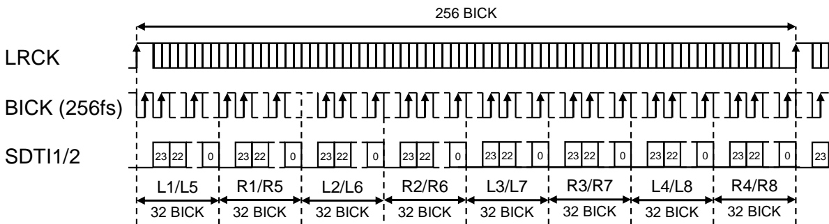
Figure 34. Mode 16 Timing
