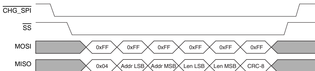
FIGURE 9-10: SPI_INVALID_REQ
