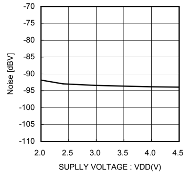
Fig.17 Output Noise (SPL)
