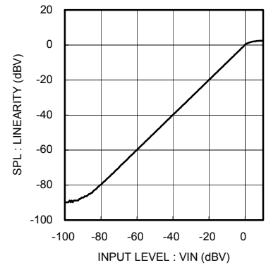
Fig.12 Linearity (SPL)
