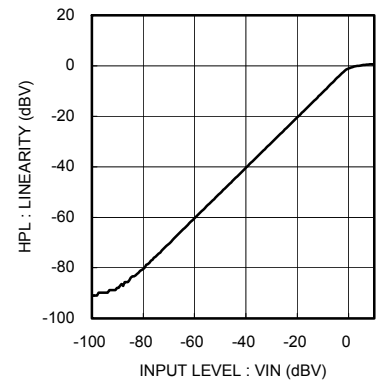
Fig.9 Linearity (HPL)
