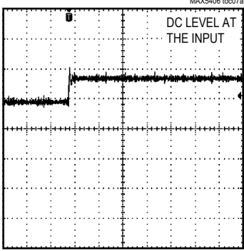
WIPER SWITCHING TRANSIENT
