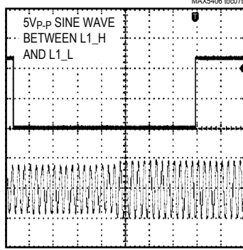
WIPER SWITCHING TRANSIENT (SUPPRESSION CIRCUIT ACTIVE)
