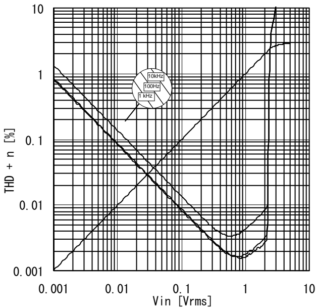
Figure 6. THD+n vs Input Voltage
