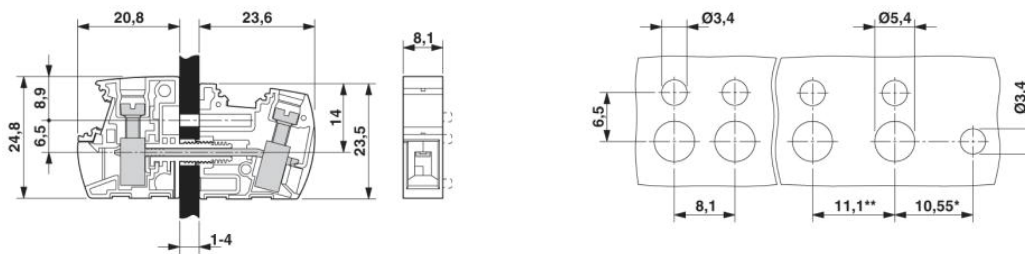
Dimensioned drawing
