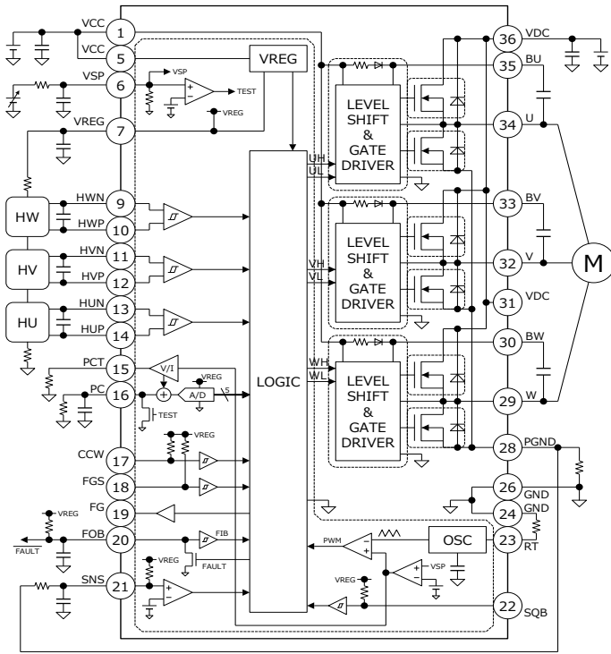
Figure 2. Block Diagram
