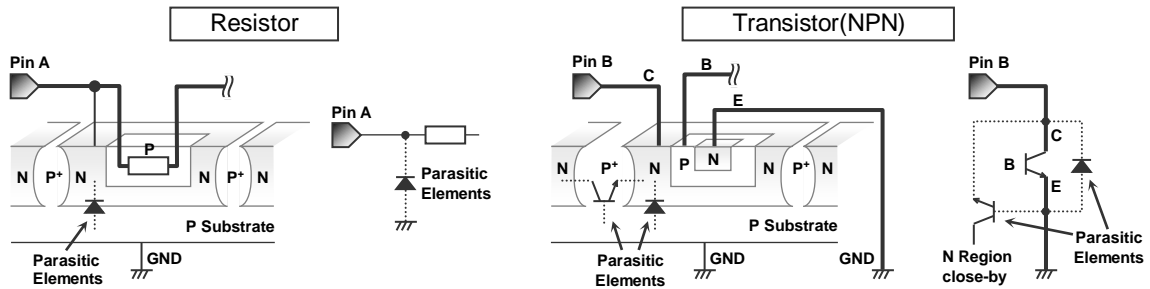
Figure 62. Example of IC structure
