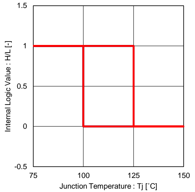
Figure 43 Thermal Shutdown
