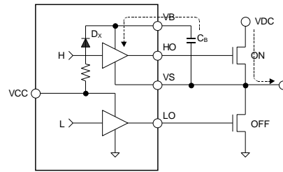
Figure 11. Discharging Period
