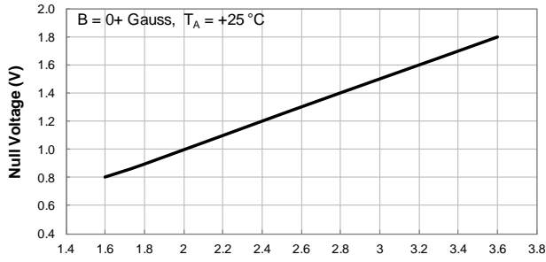
Null Voltage vs Supply Voltage
