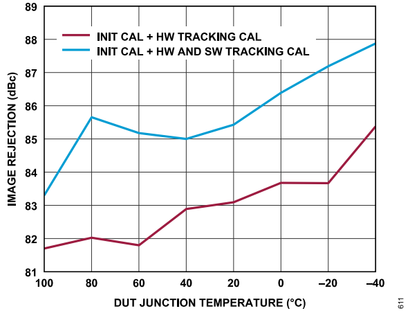
Figure 82. Receiver Image Rejection vs. DUT Junction Temperature (High to Low), Tone 1 Baseband Frequency = -5.1 MHz, Tone 2 Baseband Frequency = 13.9 MHz, ADC = Low Power, P_{OUT} = -11.1 dBFS
