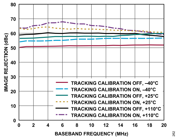
Figure 170. Transmitter Image Rejection vs. Baseband Frequency, Tracking Calibration On vs. Tracking Calibration Off, Transmitter Attenuation Code = 0
