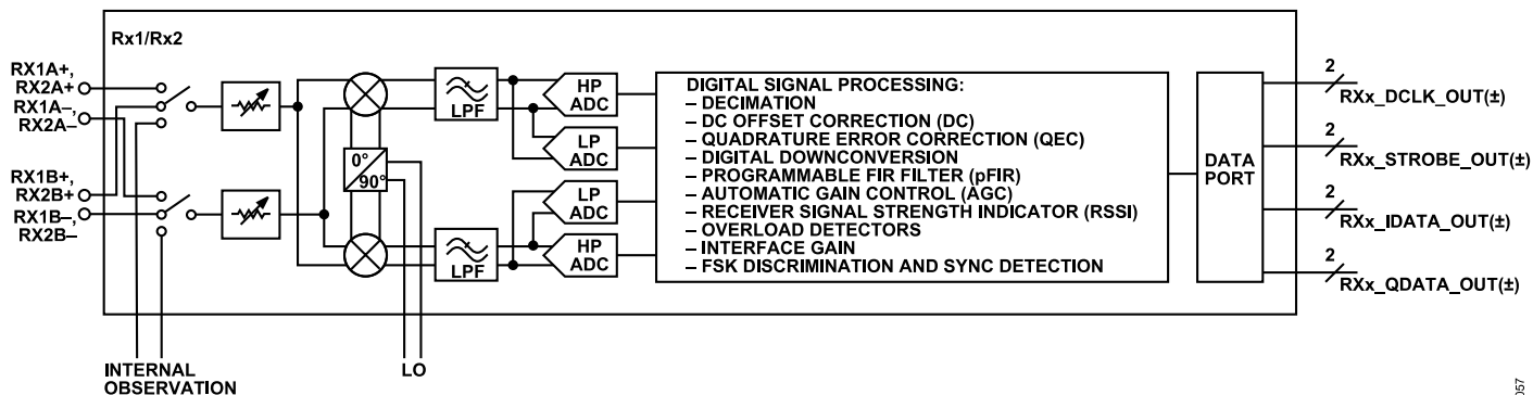
Figure 361. Receiver Architecture
