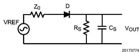
FIGURE 2. Diode Detector
