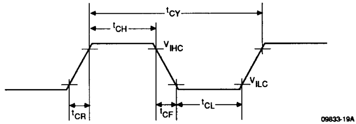
Figure 14b. External Clock
