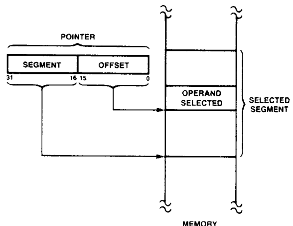
FIGURE 4. TWO COMPONENT ADDRESS
