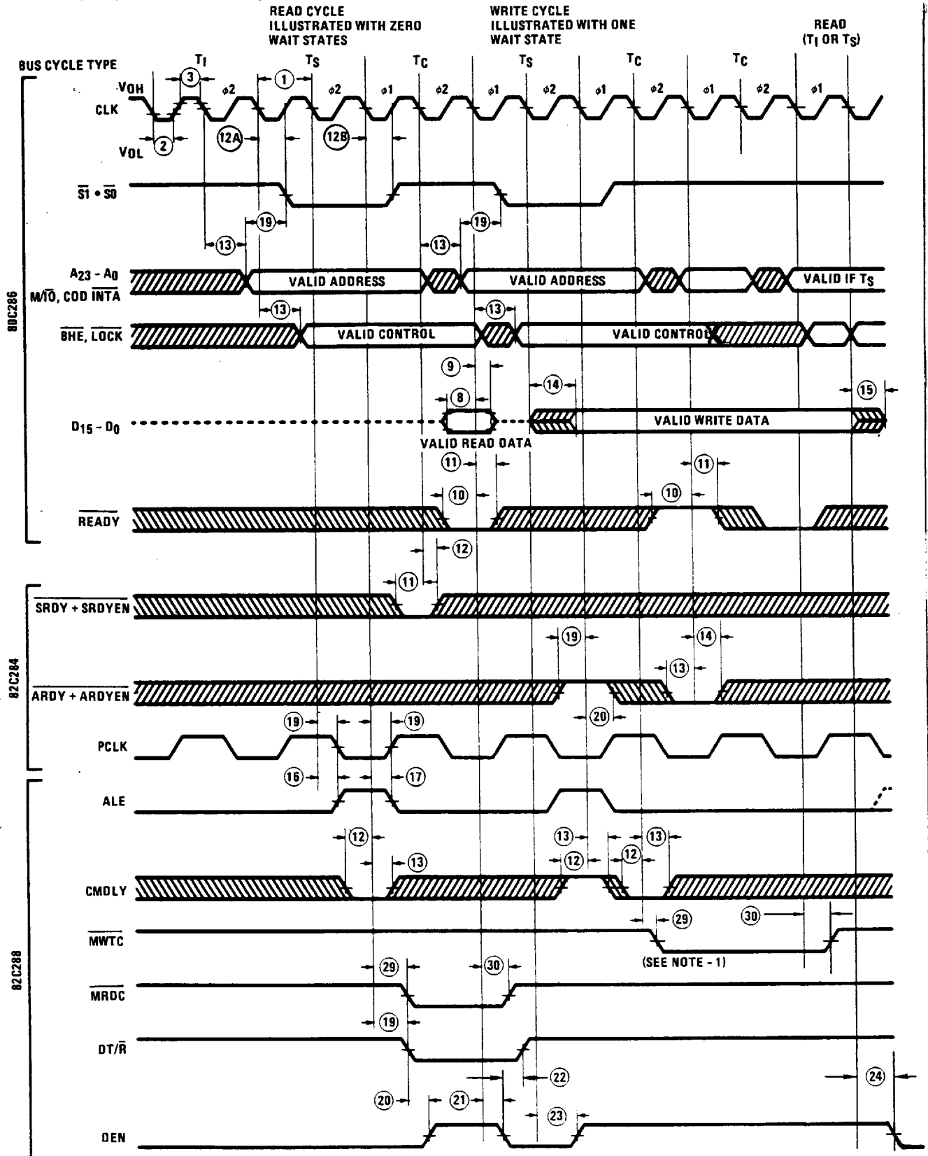
MAJOR CYCLE TIMING
