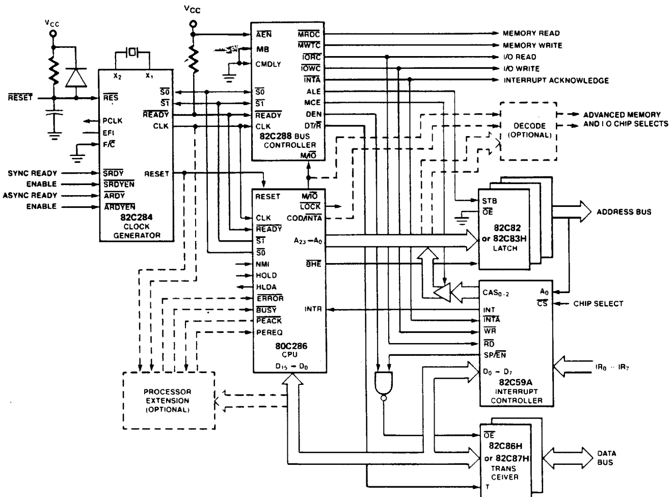
FIGURE 31. BASIC 80C286 SYSTEM CONFIGURATION
