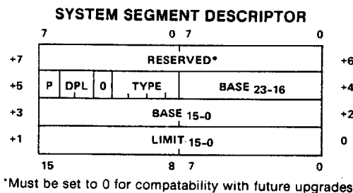
SYSTEM SEGMENT DESCRIPTOR FIELDS
