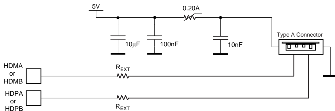
Figure 41-4. Board Schematic to Interface UHP Device Controller
