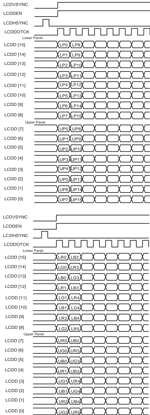
Figure 43-10. Dual Scan Monochrome and Color 16-bit Panel Timing (First Line Expanded View)
