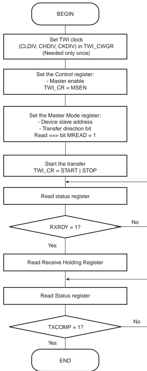
Figure 32-16. TWI Read Operation with Single Data Byte without Internal Address
