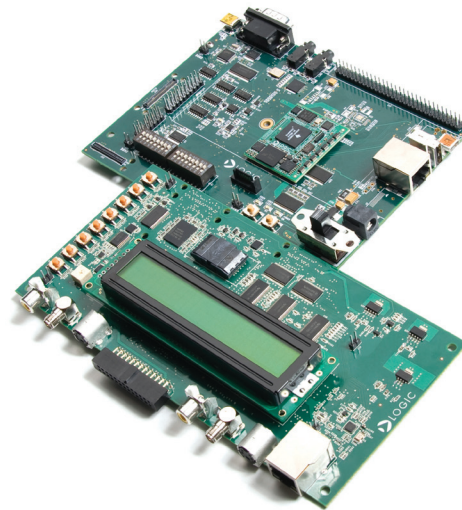
ZOOM OMAP-L138 EVM DEVELOPMENT KIT
