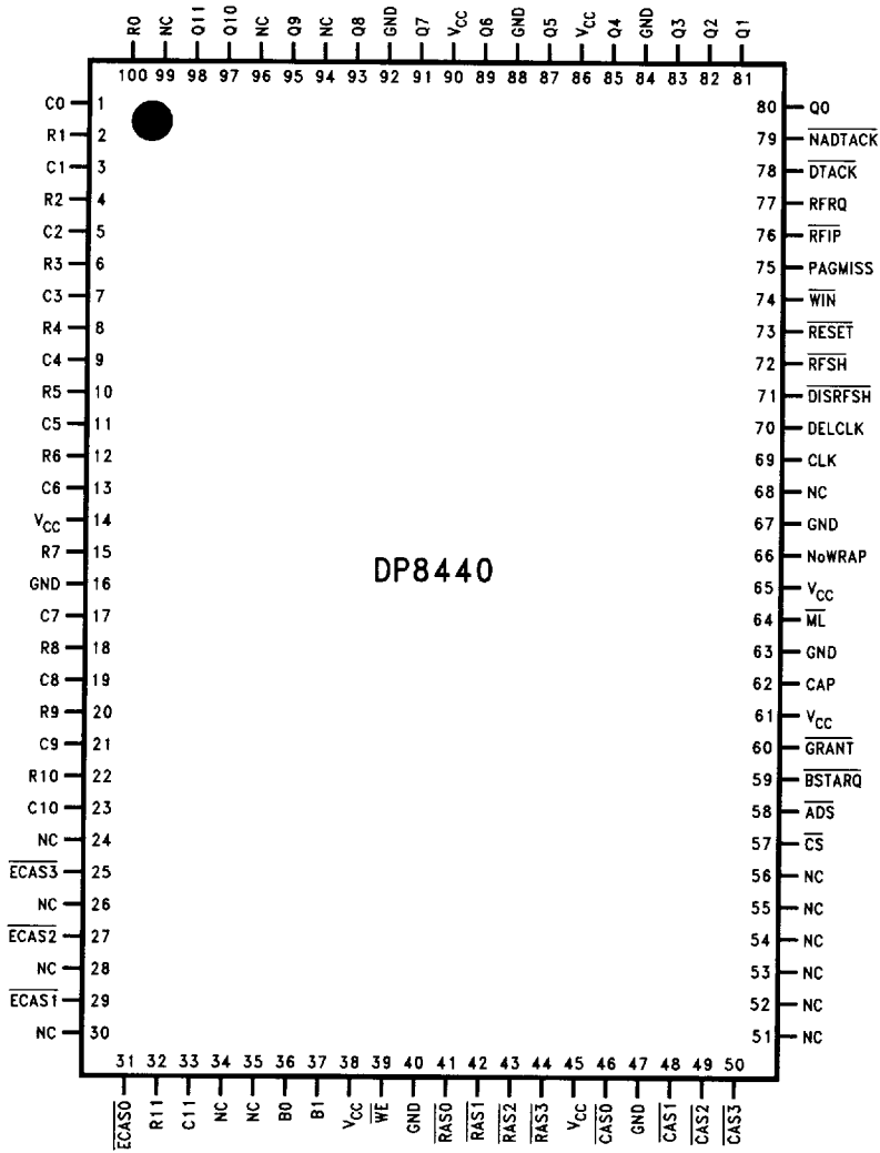
Top View
