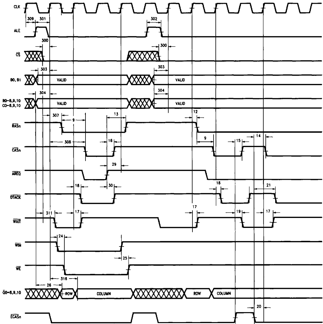
FIGURE 40. 300: Mode 0 Timing
