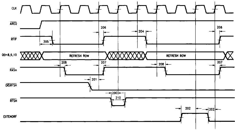
FIGURE 39. 200: Refresh Timing
