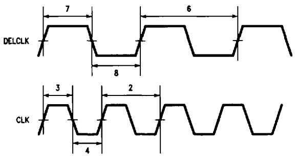
FIGURE 36. Clock, DELCLK Timing
