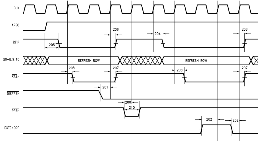
FIGURE 37. 200: Refresh Timing
