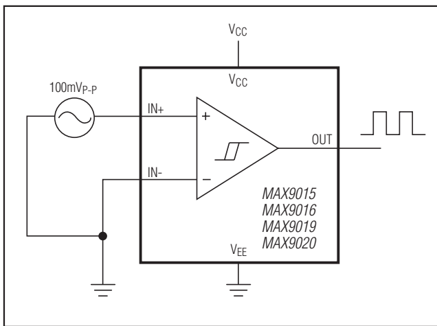
Figure 5. Zero-Crossing Detector
