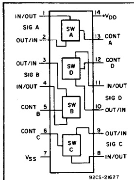
Quad Bilateral Switch
