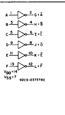
Hex Inverter
