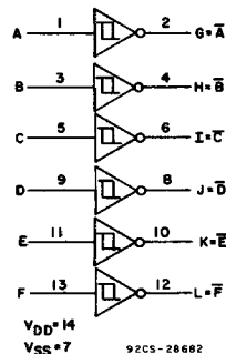
Hex Schmitt Trigger CD40106B (File No. 1017)
