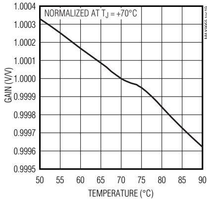
TERMINATOR GAIN vs. TEMPERATURE
