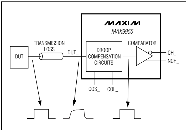
Figure 4. Cable-Droop Compensation
