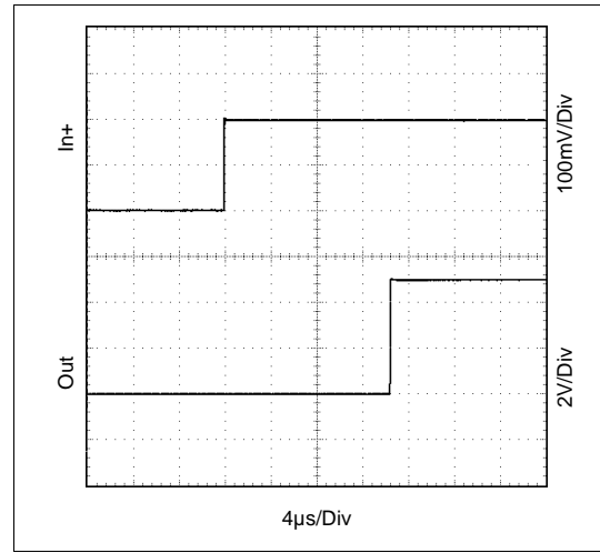
Figure 18. t_{PD+} 3V
