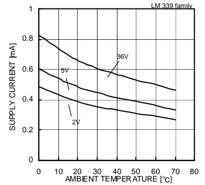
Fig.23 Supply Current - Ambient Temperature
