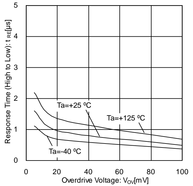
Figure 37. Response Time (High to Low) vs Overdrive Voltage (V CC =5 V, V RL =5 V, R L =5.1 kΩ)
