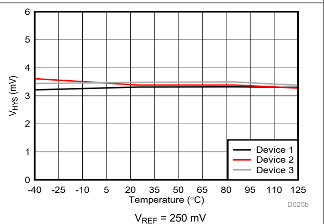
Figure 6-28. Cmp0 Trip Threshold Hysteresis vs Temperature
