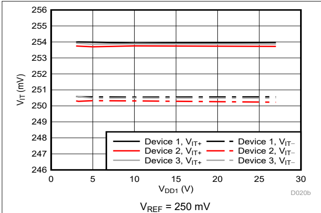
Figure 6-23. Cmp0 Trip Threshold vs Supply Voltage
