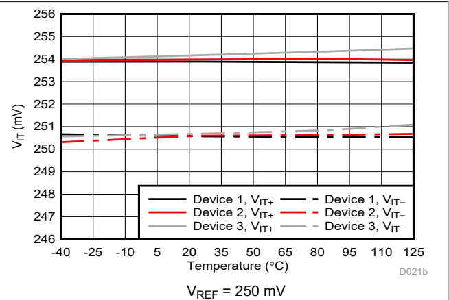
Figure 6-24. Cmp0 Trip Threshold vs Temperature
