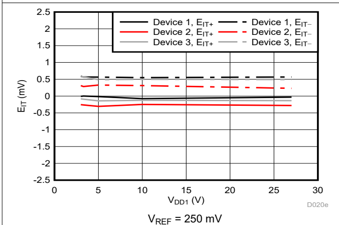
Figure 6-25. Cmp0 Trip Threshold Error vs Supply Voltage
