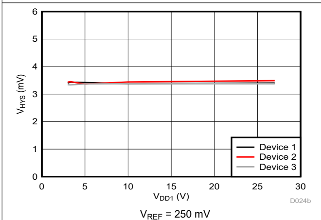
Figure 6-27. Cmp0 Trip Threshold Hysteresis vs Supply Voltage
