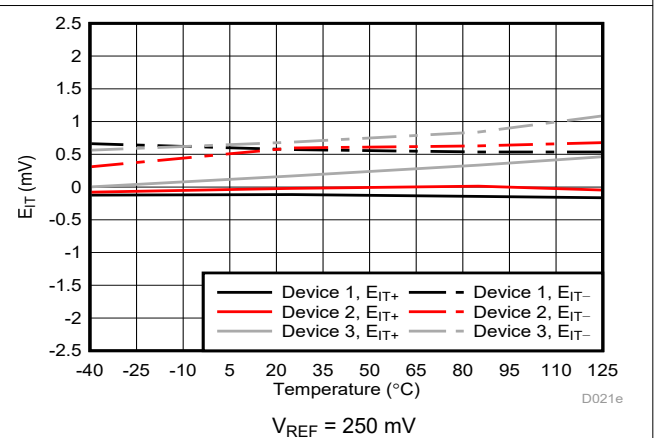
Figure 6-26. Cmp0 Trip Threshold Error vs Temperature
