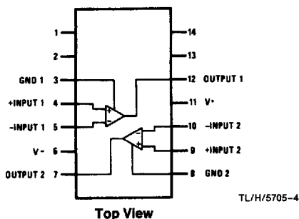
Dual-In-Line-Package
