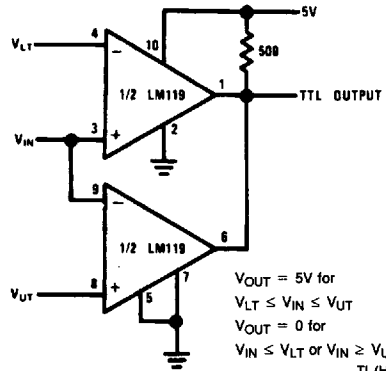
Window Detector
