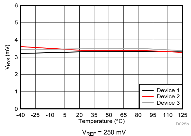
Figure 6-16. Trip Threshold Hysteresis vs Temperature
