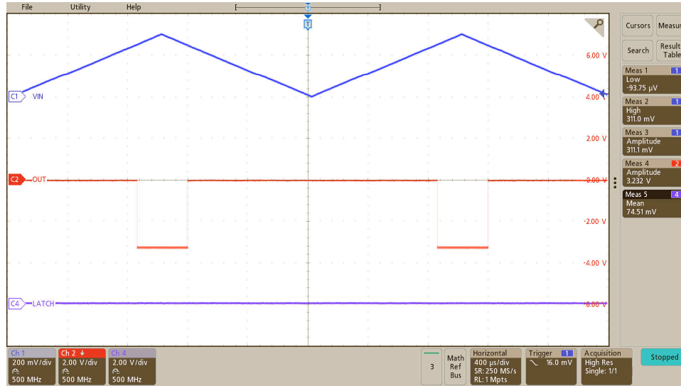
Figure 8-2. Output Response of the AMC22C11 to a Triangular Input Waveform
