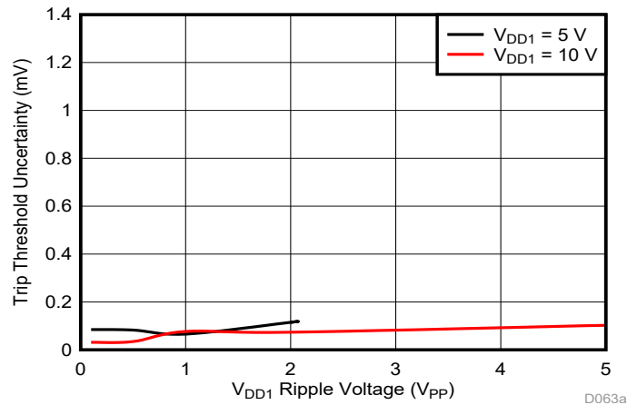
Figure 8-3. Trip Threshold Sensitivity to VDD1 Ripple Voltage (f RIPLLE = 10 kHz)
