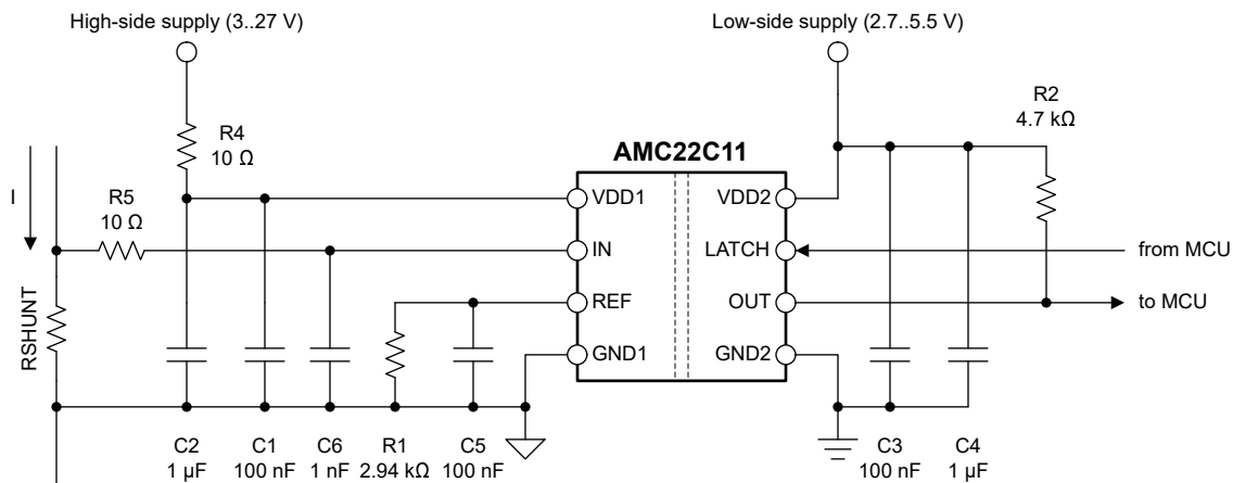
Figure 8-4. Decoupling of the AMC22C11
