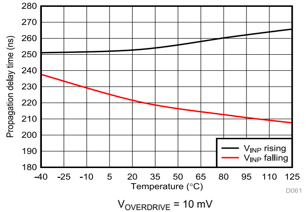
Figure 6-24. Propagation Delay vs Temperature
