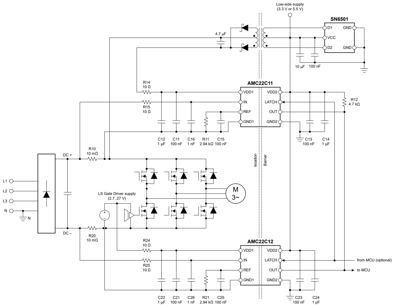
Figure 8-1. Using the AMC22C11 for DC+ Overcurrent Detection
