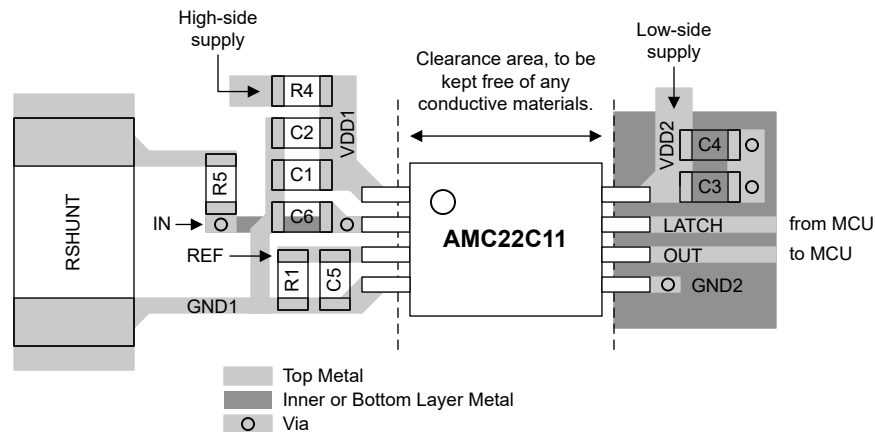
Figure 8-5. Recommended Layout of the AMC22C11
