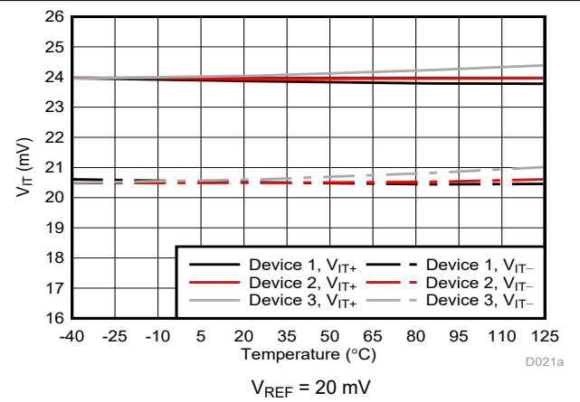
Figure 6-6. Cmp0 Trip Threshold vs Temperature
