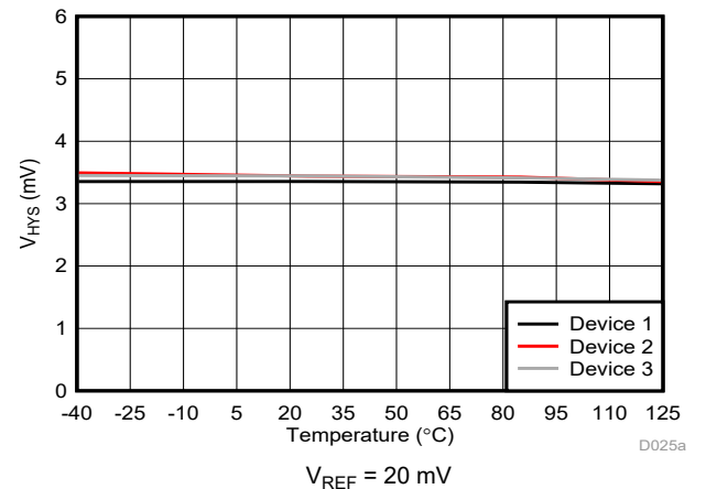
Figure 6-10. Cmp0 Trip Threshold Hysteresis vs Temperature
