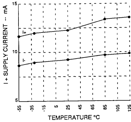
Supply Currents vs Temperature
