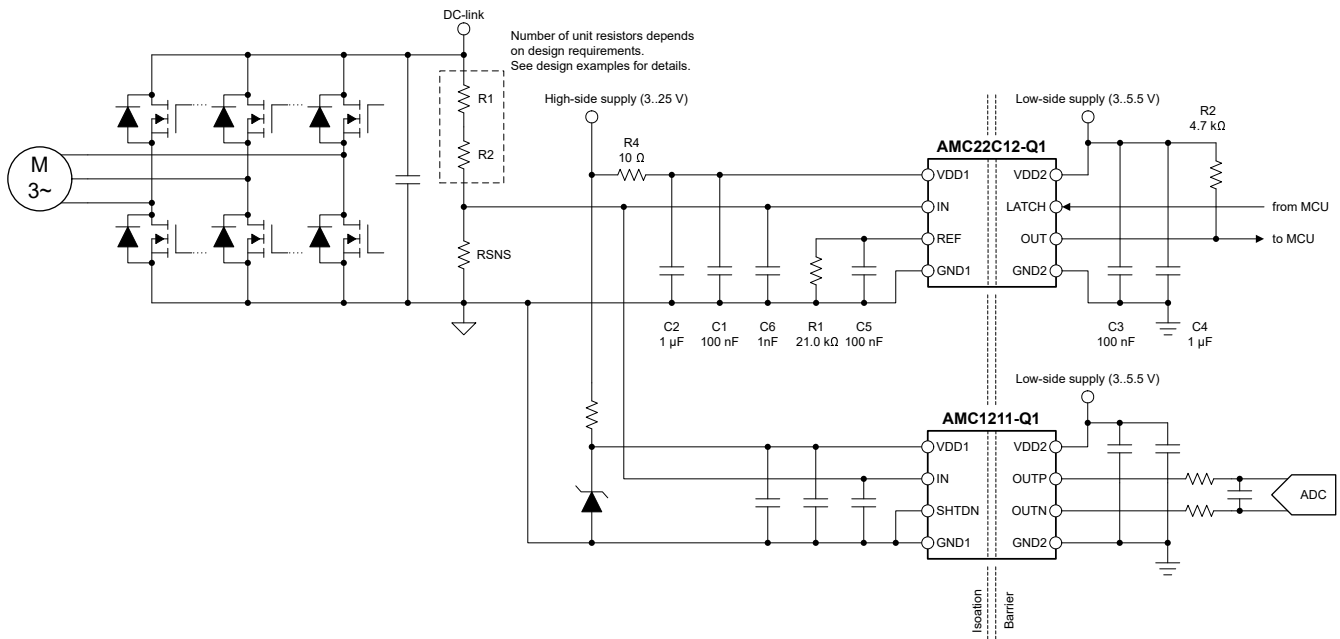
Figure 8-2. Using the AMC22C12-Q1 for Overvoltage Detection
