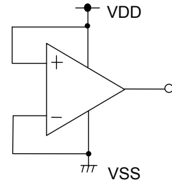
Figure 29. Example of Application Circuit for Unused Comparator
