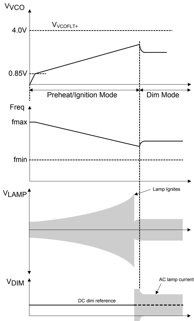
Figure 3, Preheat/Ignition/Dim Mode timing diagram.
