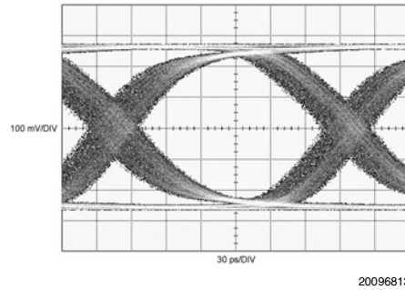
FIGURE 6. Typical 5Gb/s Equalizer Output Signal, with Input as shown in Figure 5
