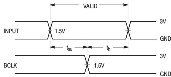
Figure 11. Setup/Hold Times
