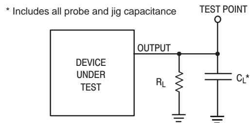
Figure 12. Test Circuit
