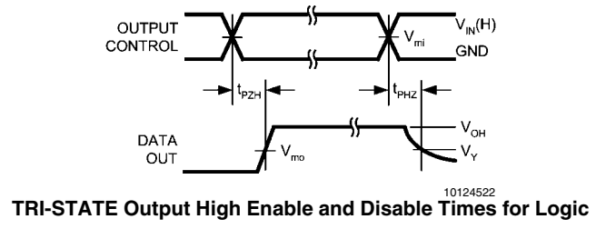
Waveform for Inverting and Non-inverting Functions
