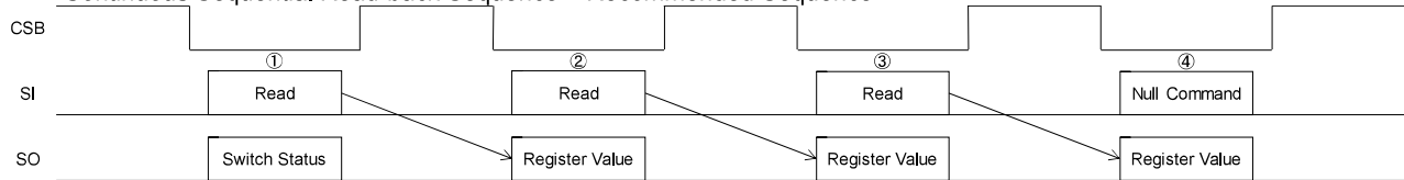
Figure 12. Continuous Read-back Sequence
