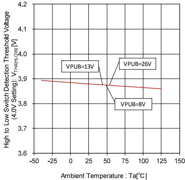
Figure 77. High to Low Switch Detection Threshold Voltage - Temperature Characteristic (4.0V Setting)
