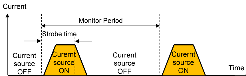
Figure 13. Intermittent Monitoring
