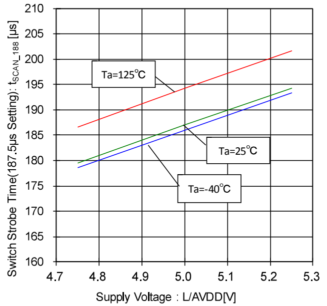
Figure 114. Switch Strobe Time- Voltage Characteristic (187.5µsSetting)
