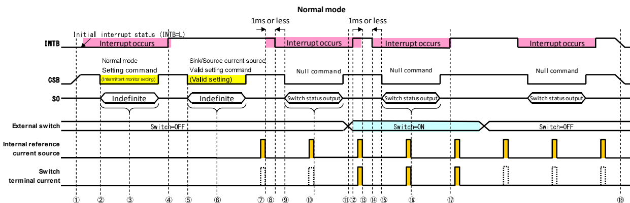
Figure 8. Basic Operation 2
