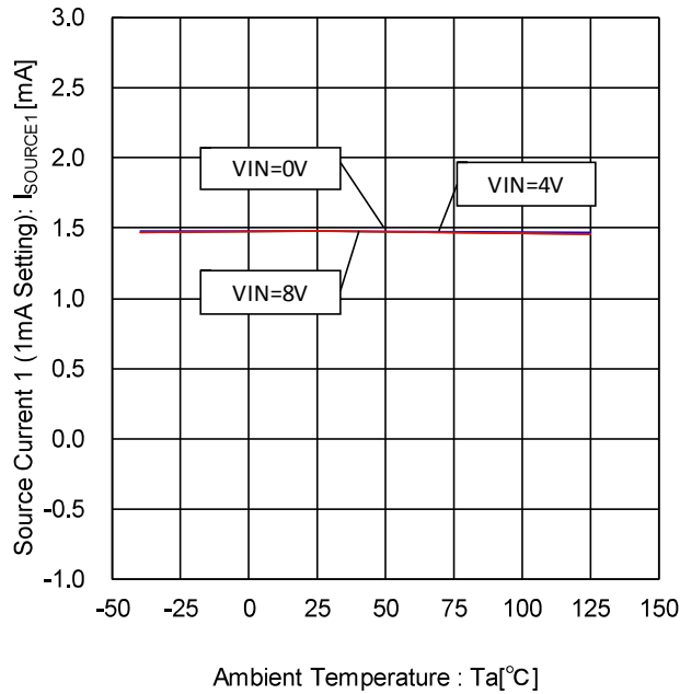
Figure 33. Source Current 1- Temperature Characteristic (1mA Setting)
