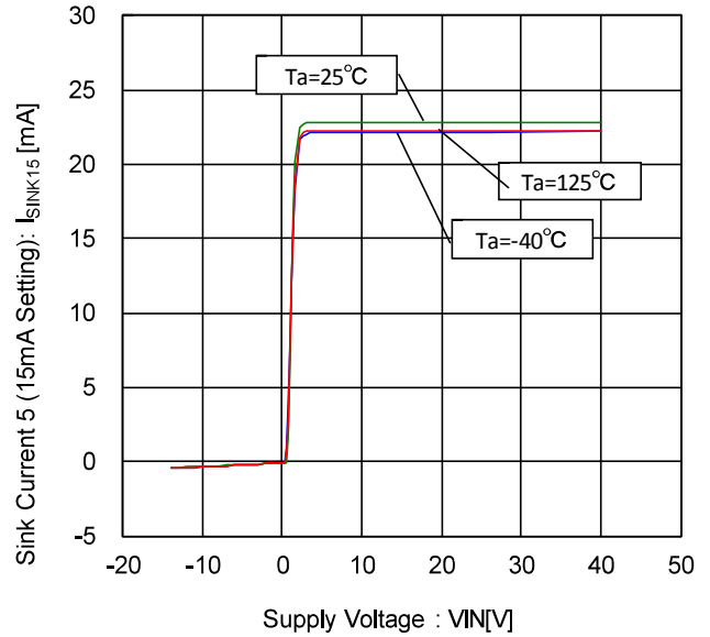
Figure 70. Sink Current 5- Voltage Characteristic (15mA Setting)
