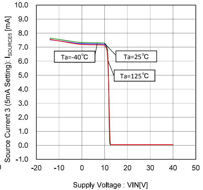
Figure 50. Source Current 3- Voltage Characteristic (5mA Setting)
