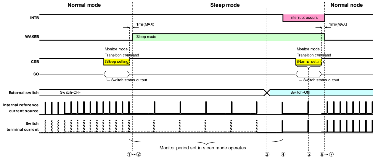
Figure 9. Basic Operation 3
