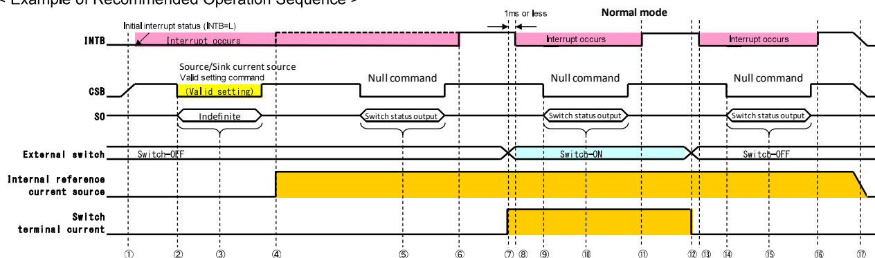
Figure 7. Basic Operation 1
