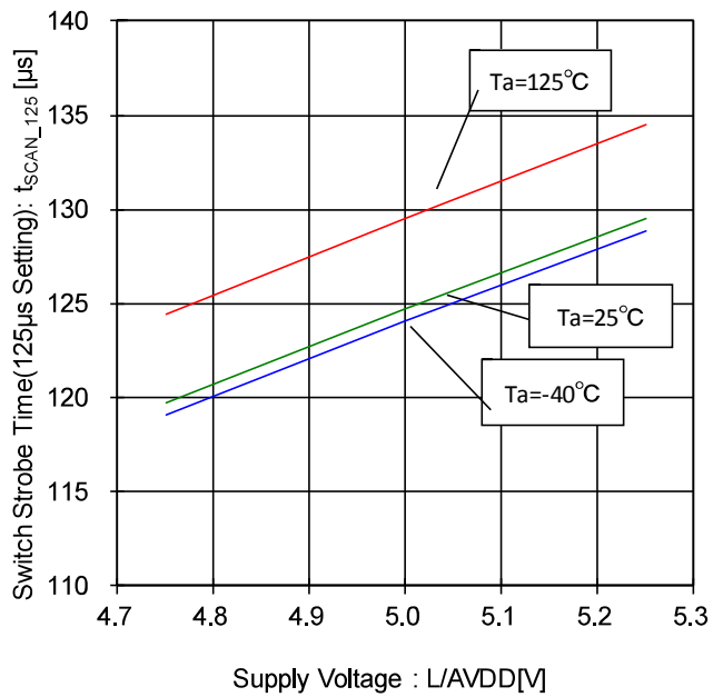
Figure 112. Switch Strobe Time- Voltage Characteristic (125µs Setting)
