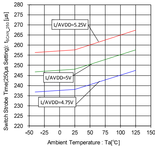
Figure 115. Switch Strobe Time- Temperature Characteristic (250µs Setting)
