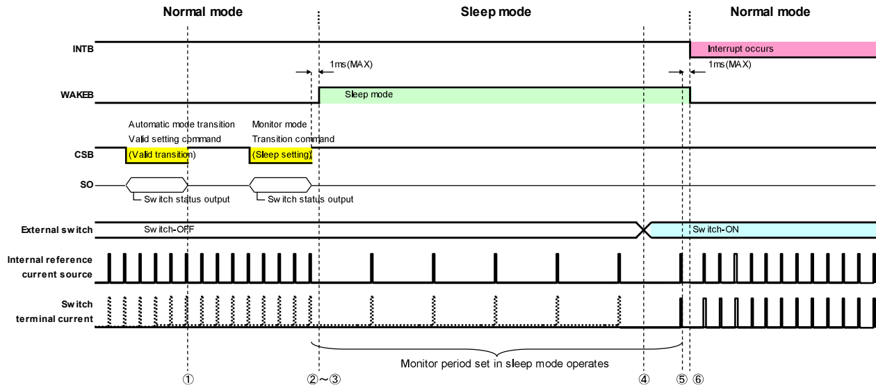
Figure 10. Basic Operation 4
