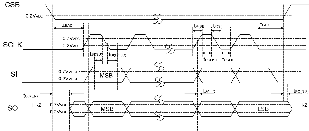
Figure 4. Serial Access Timing
