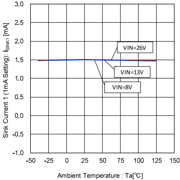
Figure 37. Sink Current 1- Temperature Characteristic (1mA Setting)
