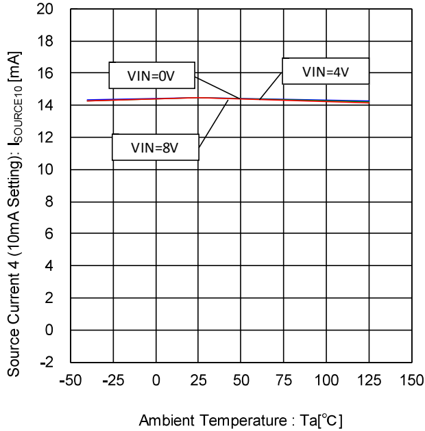
Figure 57. Source Current 4- Temperature Characteristic (10mA Setting)
