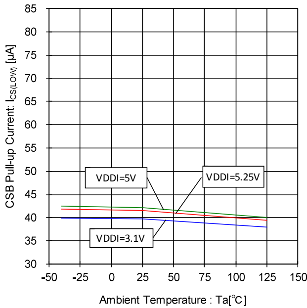
Figure 83. CSB Pull-up Current- Temperature Characteristic (CSB=0V)
