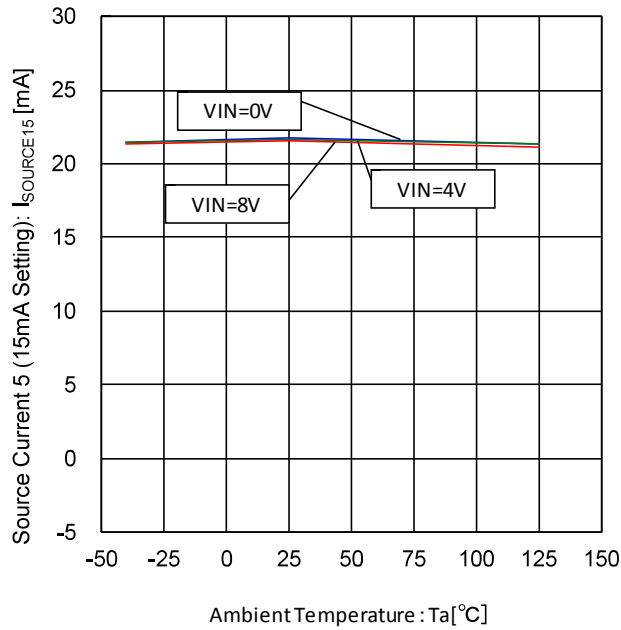
Figure 65. Source Current 5- Temperature Characteristic (15mA Setting)
