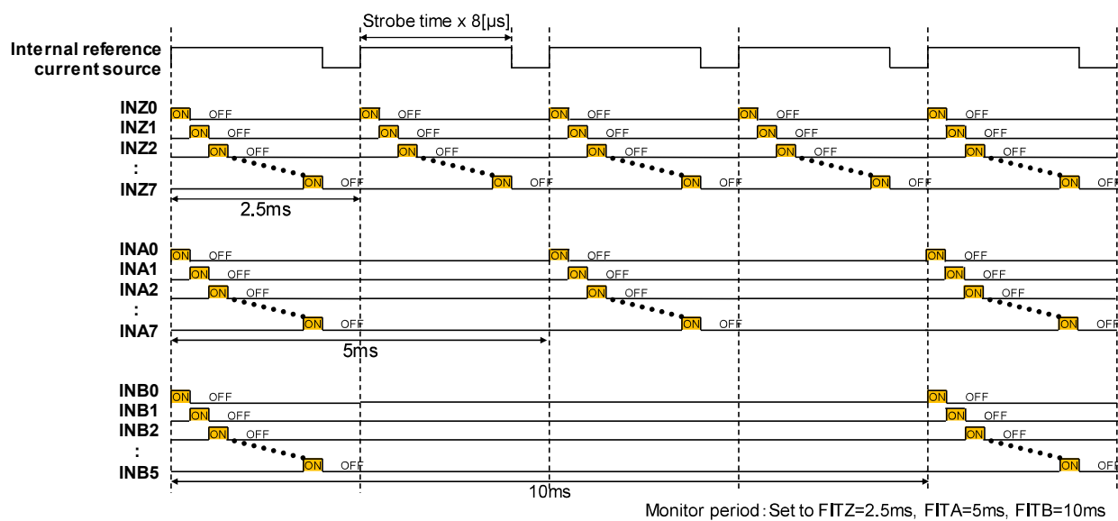
Figure 15. Sequential Monitoring by Power Supply System Example
