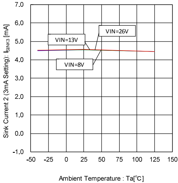
Figure 45. Sink Current 2- Temperature Characteristic (3mA Setting)
