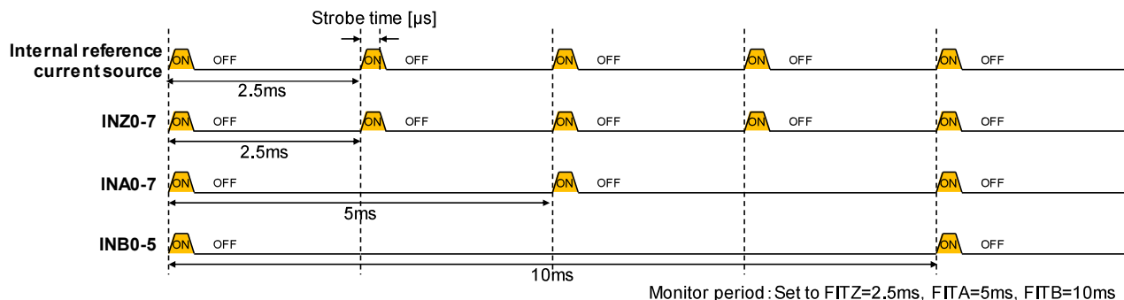
Figure 14. Intermittent Monitoring at the Same Time Example
