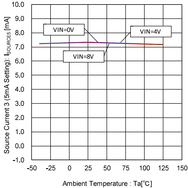
Figure 49. Source Current 3- Temperature Characteristic (5mA Setting)
