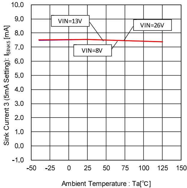
Figure 53. Sink Current 3- Temperature Characteristic (5mA Setting)
