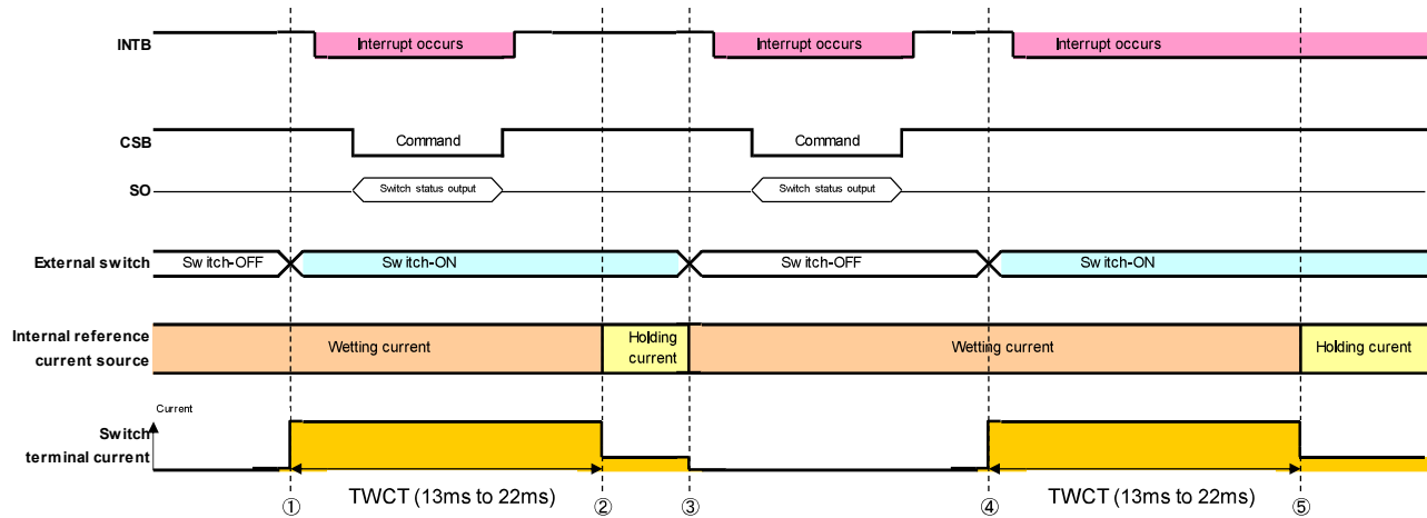
Figure 17. Wetting Current Timer (Continuous Operation)
