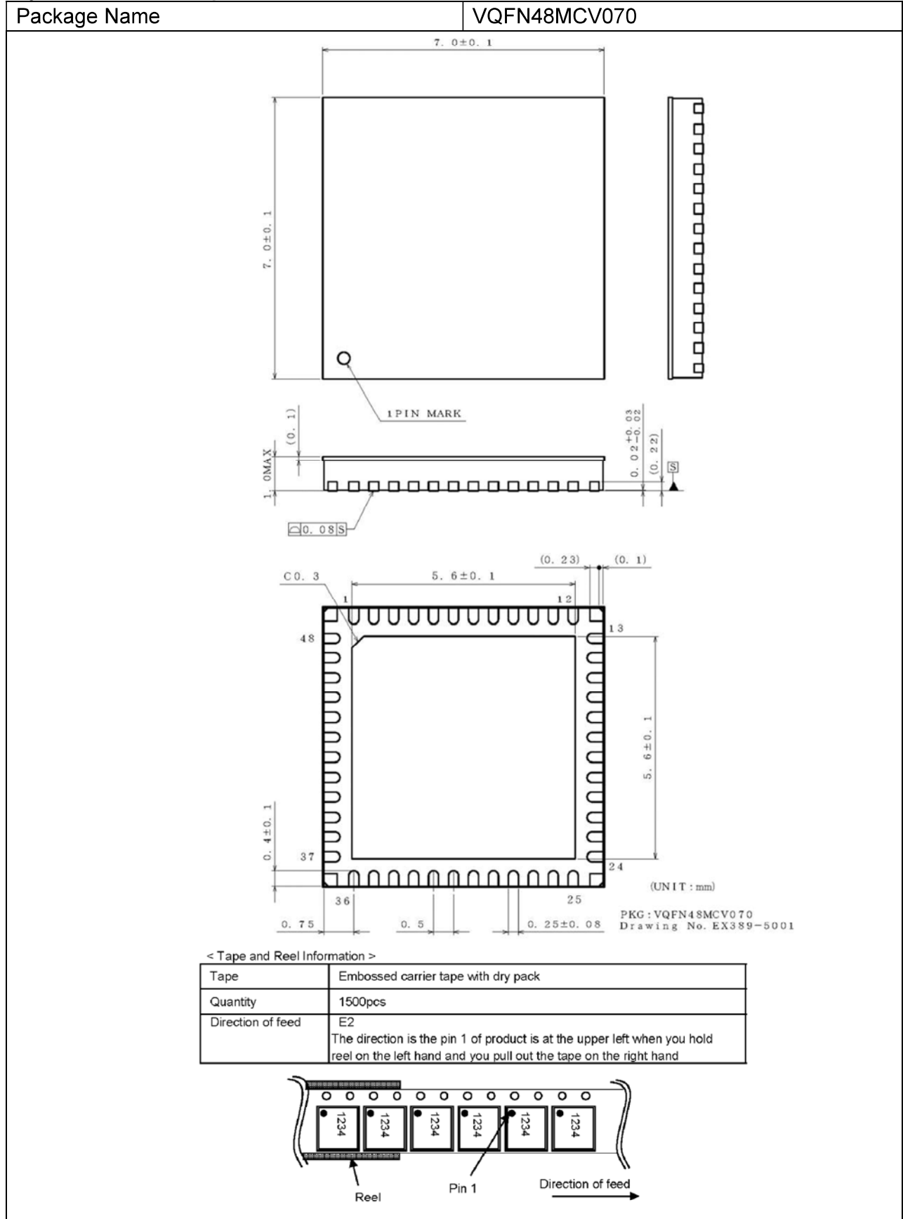
Figure 126. Physical Dimensions, Tape and Reel information
