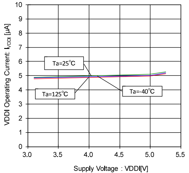
Figure 28. VDDI Operating Current- Voltage Characteristic (INTB="H", CSB="H")
