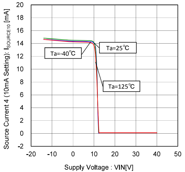
Figure 58. Source Current 4- Voltage Characteristic (10mA Setting)
