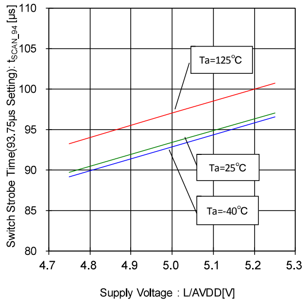
Figure 110. Switch Strobe Time- Voltage Characteristic (93.75µs Setting)
