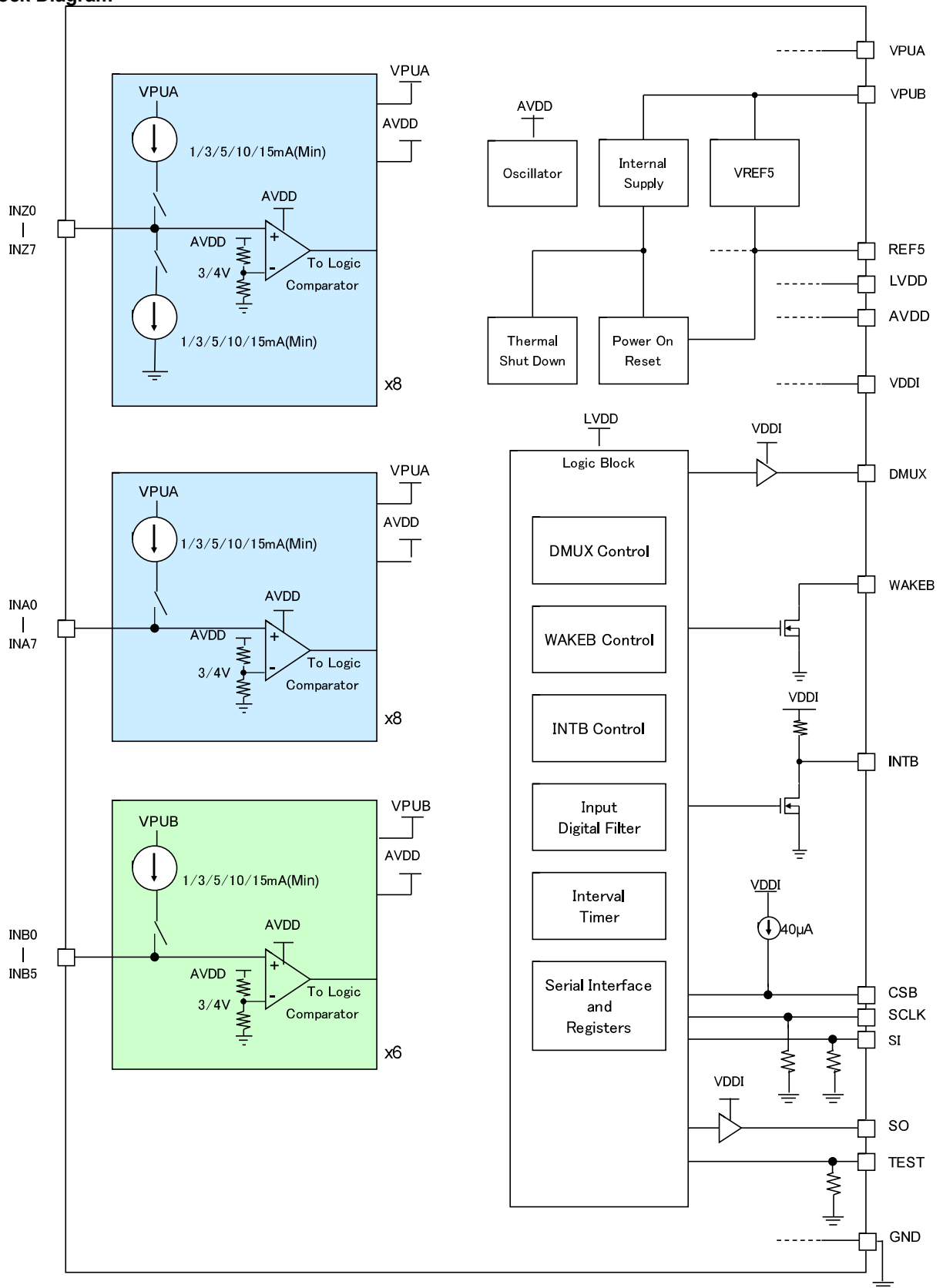
Figure 3. Block Diagram
