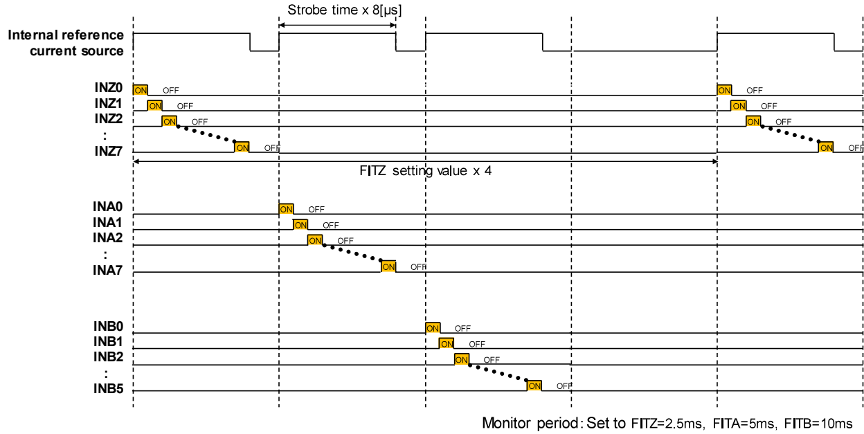
Figure 16. Sequential Monitoring of All Switches Terminals Example
