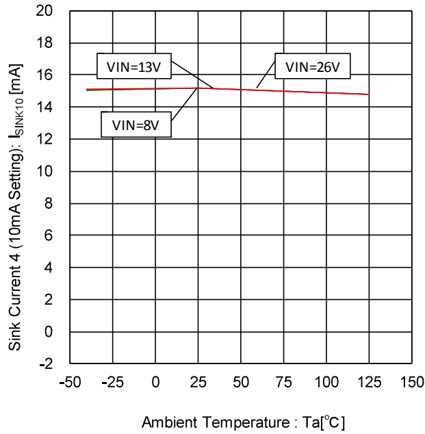
Figure 61. Sink Current 4- Temperature Characteristic (10mA Setting)
