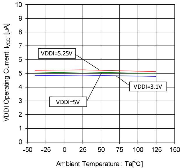
Figure 27. VDDI Operating Current- Temperature Characteristic (INTB="H", CSB="H")
