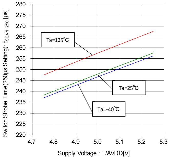
Figure 116. Switch Strobe Time- Voltage Characteristic (250µs Setting)
