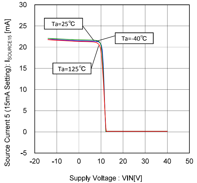
Figure 66. Source Current 5- Voltage Characteristic (15mA Setting)
