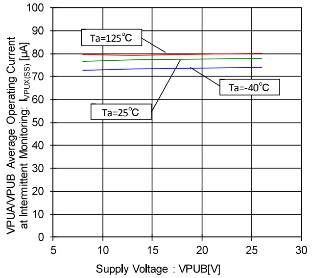
Figure 26. VPUA/VPUB Average Operating Current at Intermittent Monitoring - Voltage Characteristic (Monitoring Period: 50ms, Strobe Time: 125µs, Source/Sink Current Setting: 1mA)
