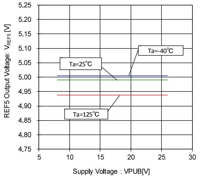
Figure 30. REF5 Output Voltage- Voltage Characteristic
