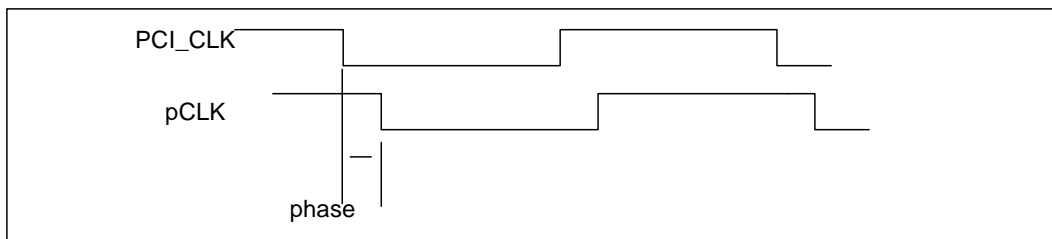
Figure 3-7. Phase Offset in Clock Slave Mode – Frequencies ≤ 33 MHz
