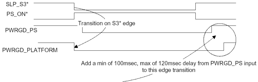
Figure 7.12 – PRWGD_PLATFORM Generation
