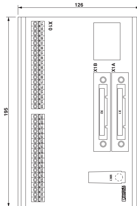
Dimensional drawing
