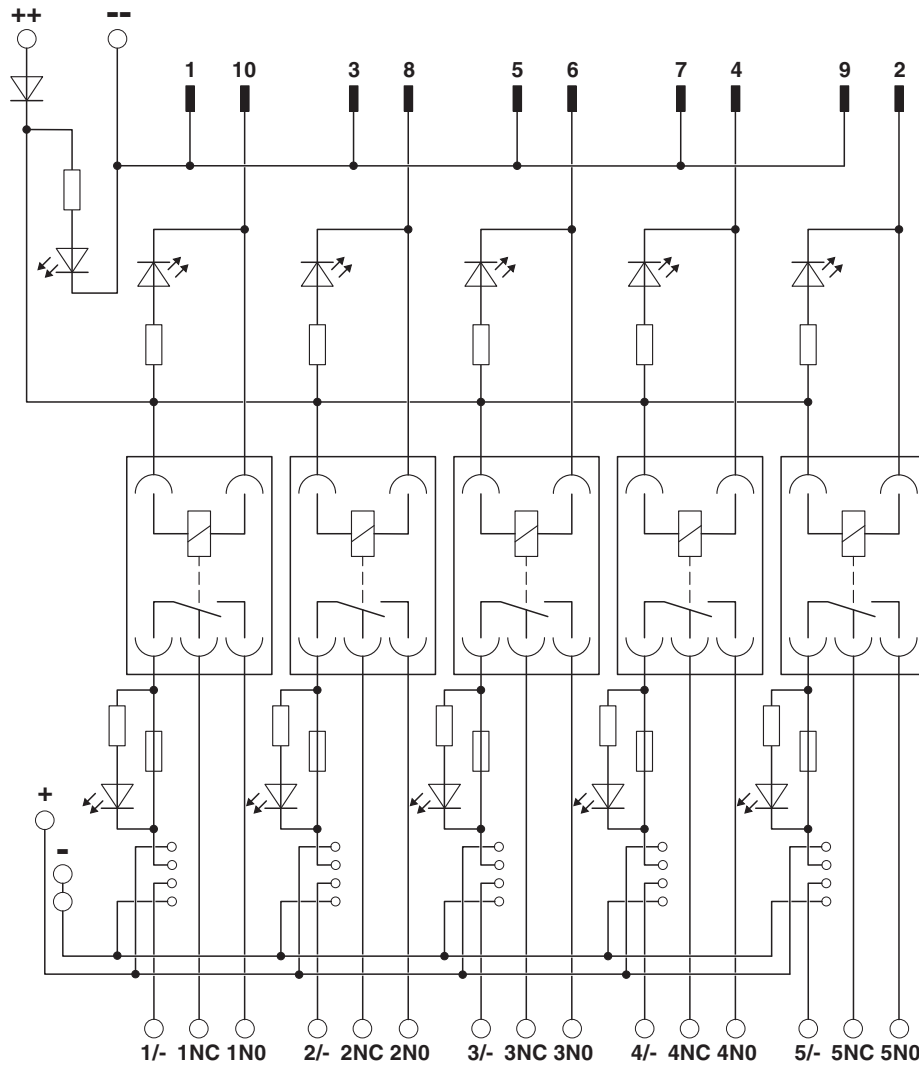
Circuit diagram
