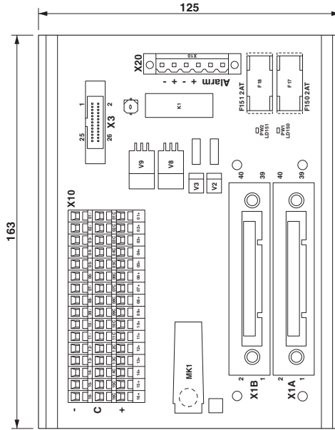
Dimensional drawing
